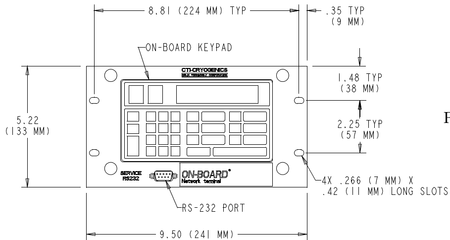
Figure 1-2: Network Terminal Dimensions (48 VDC Configuration)
